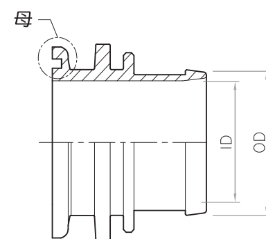
插管(10kg/cm 2 )
